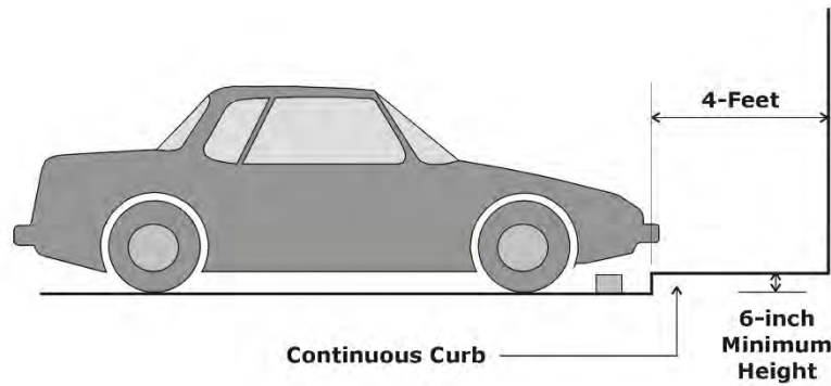
Figure 7.04-D: Continuous curbs.
