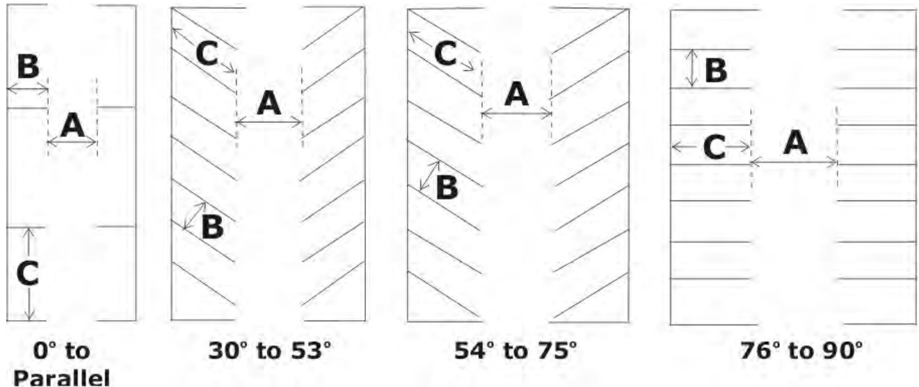
Figure 7.04-C: Parking Area Dimensions
